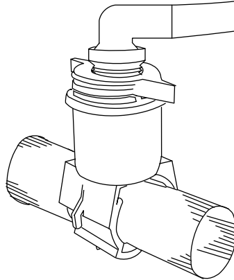
BS 12500 with Swing Pipe Fitting Application
