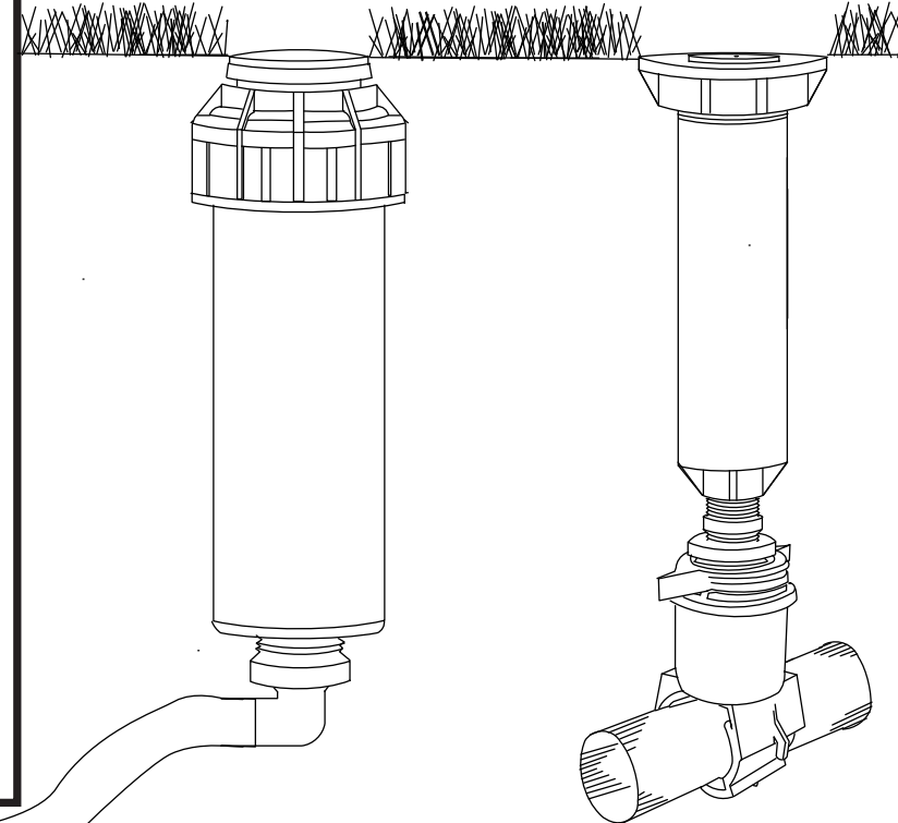
BS 12750 with 3/4" to 1/2" Riser Application
